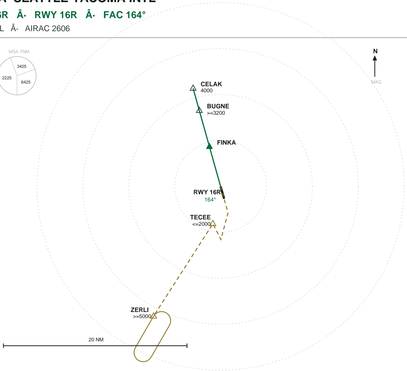
PLAN
